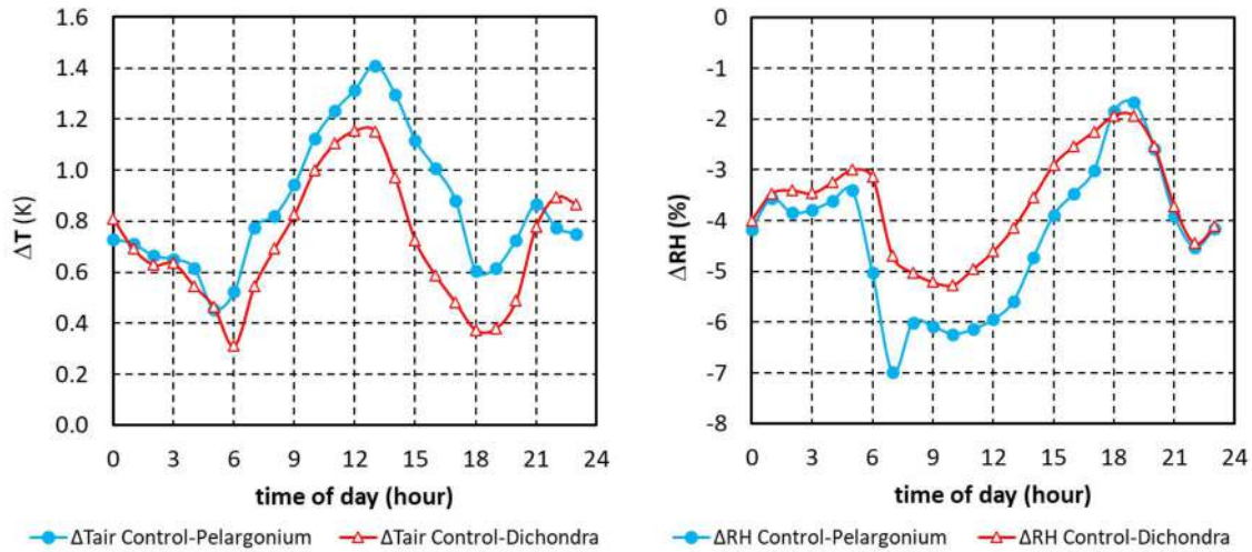
Fig 2. Left – Average diurnal profile of the difference in air temperature between the control plot and test plots. Right - Average diurnal profile of the difference in relative humidity between the control plot and test plots, for the month of August 2020.
